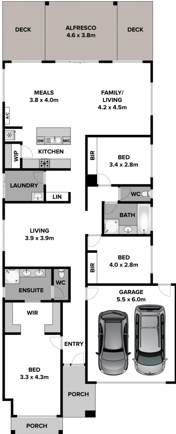
GROUND FLOOR
